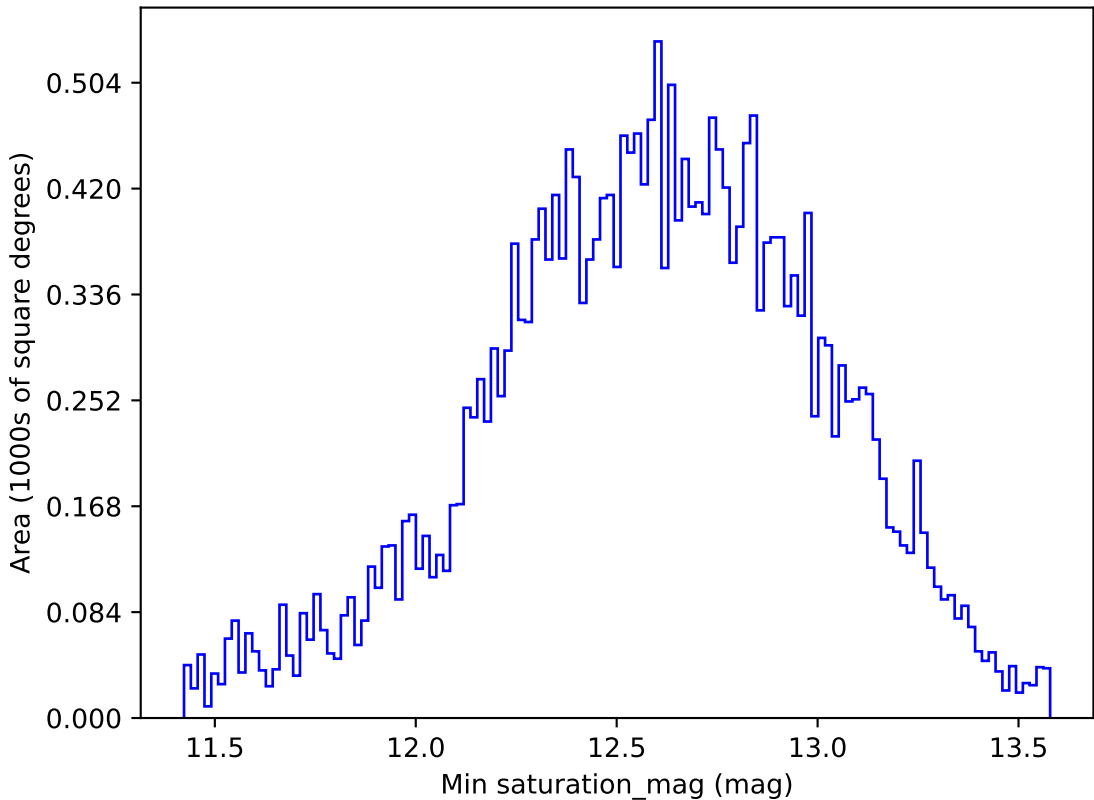
too_ignore_10_1v3.4_10yrs All sky r band: Min saturation_mag
