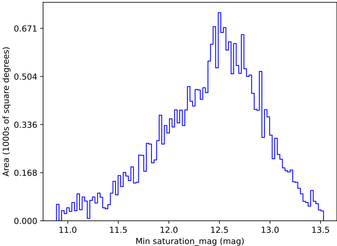
too_ignore_10_1v3.4_10yrs All sky i band: Min saturation_mag
