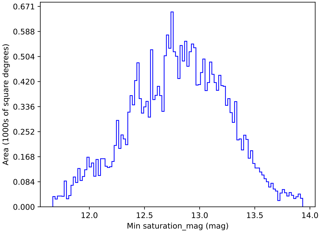
too_ignore_10_1v3.4_10yrs All sky g band: Min saturation_mag
