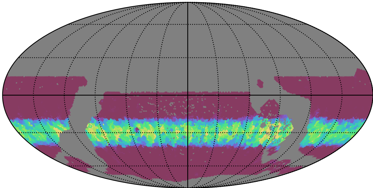
too_ignore_10_1v3.4_10yrs WFD u band: Min normairmass
