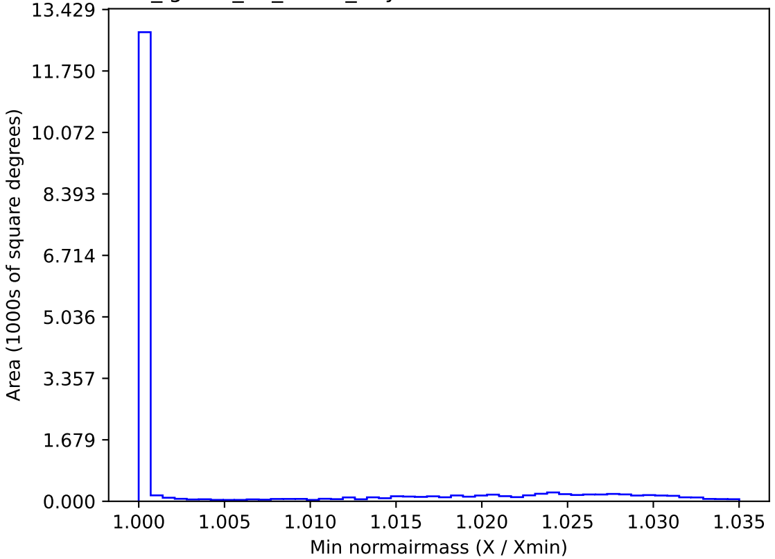
too_ignore_10_1v3.4_10yrs WFD r band: Min normairmass
