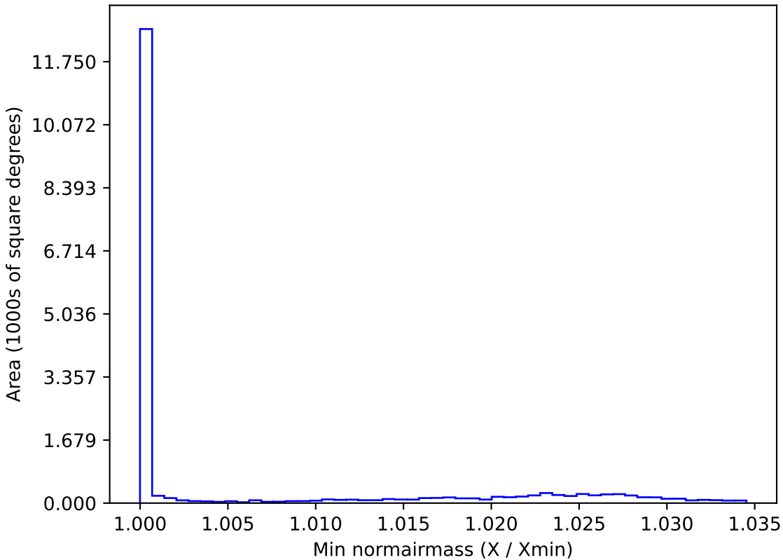
too_ignore_10_1v3.4_10yrs WFD i band: Min normairmass
