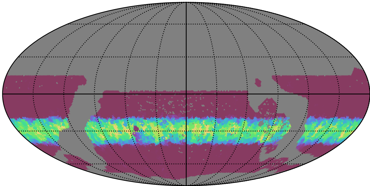
too_ignore_10_1v3.4_10yrs WFD g band: Min normairmass
