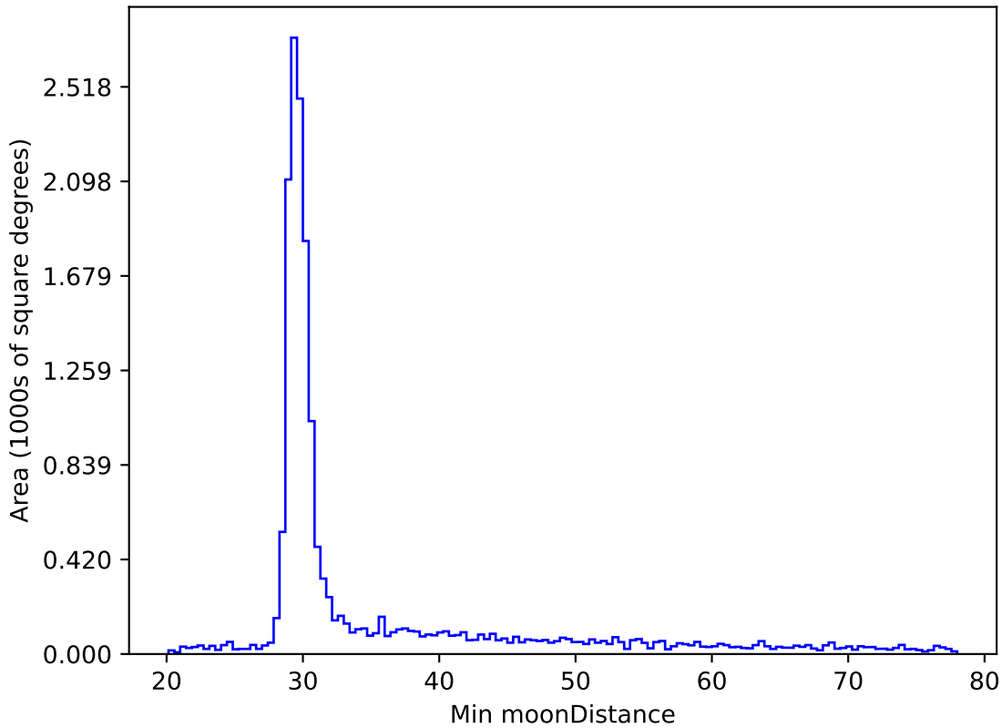
too_ignore_10_1v3.4_10yrs WFD z band: Min moonDistance
