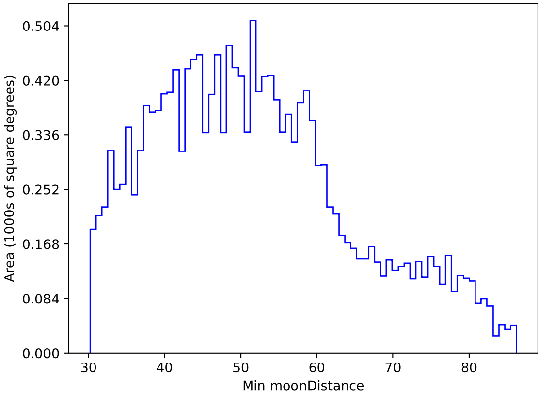
too_ignore_10_1v3.4_10yrs WFD u band: Min moonDistance
