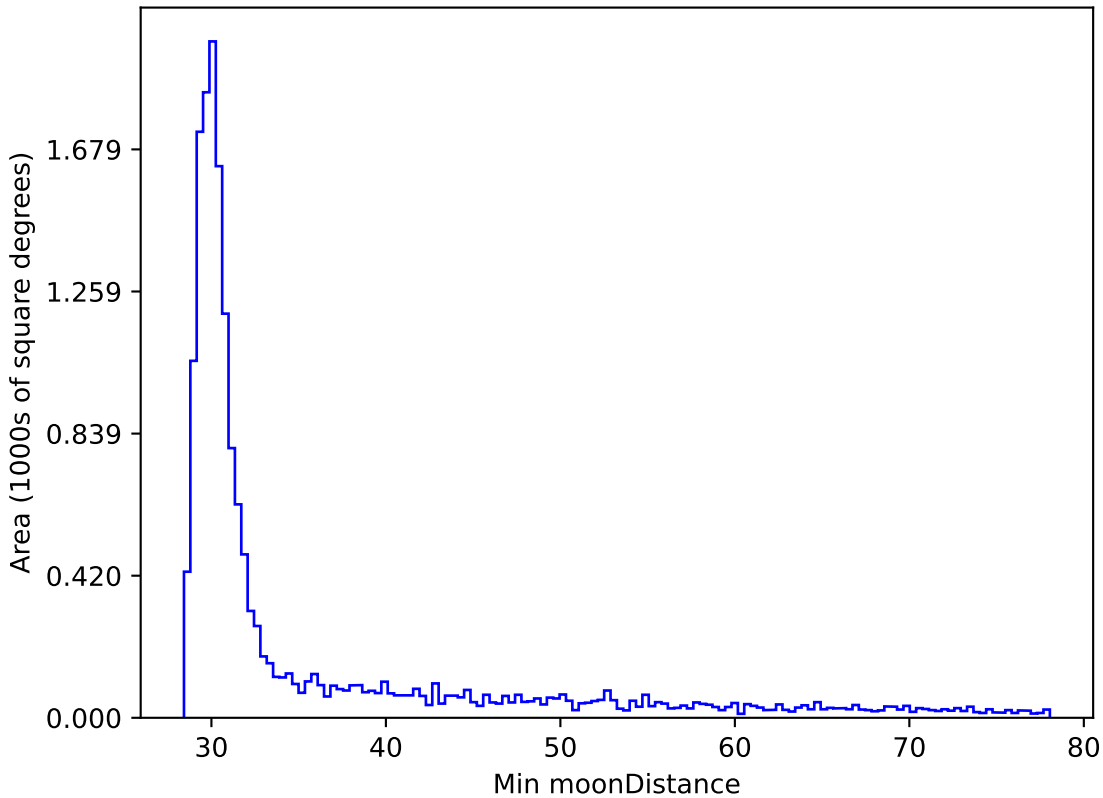
too_ignore_10_1v3.4_10yrs WFD i band: Min moonDistance
