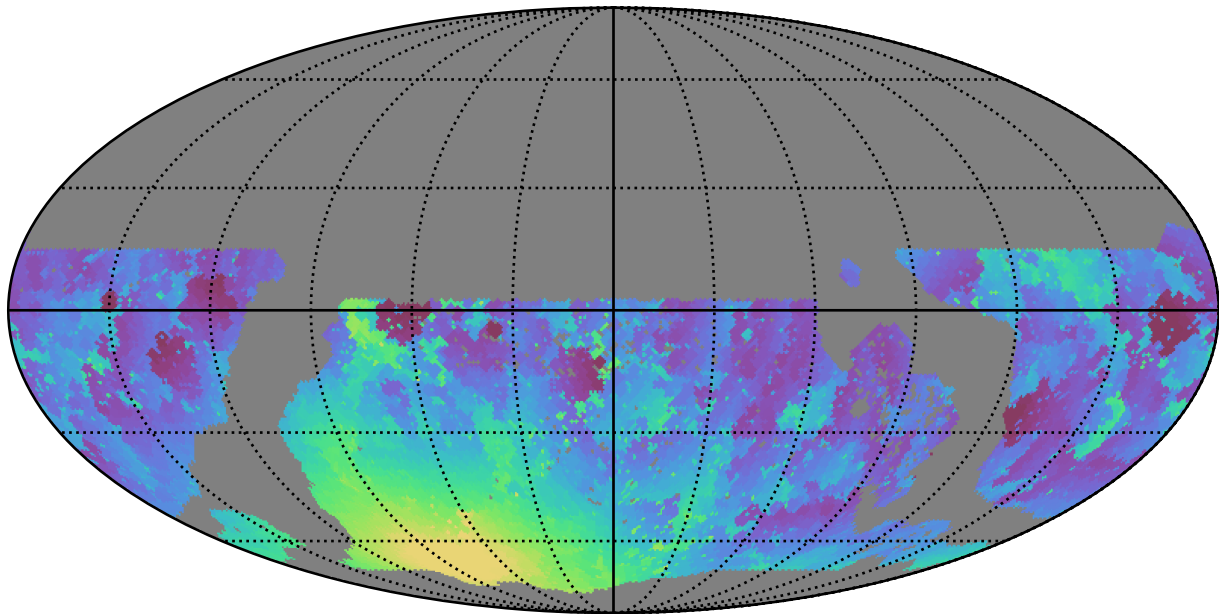
too_ignore_10_1v3.4_10yrs WFD g band: Min moonDistance
