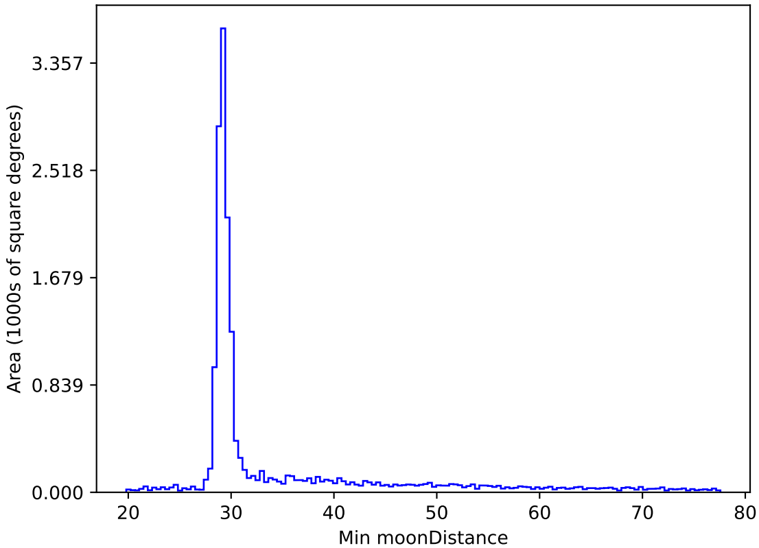
too_ignore_10_1v3.4_10yrs WFD all bands: Min moonDistance
