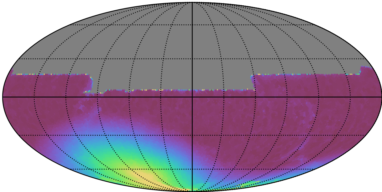
too_ignore_10_1v3.4_10yrs All sky y band: Min moonDistance
