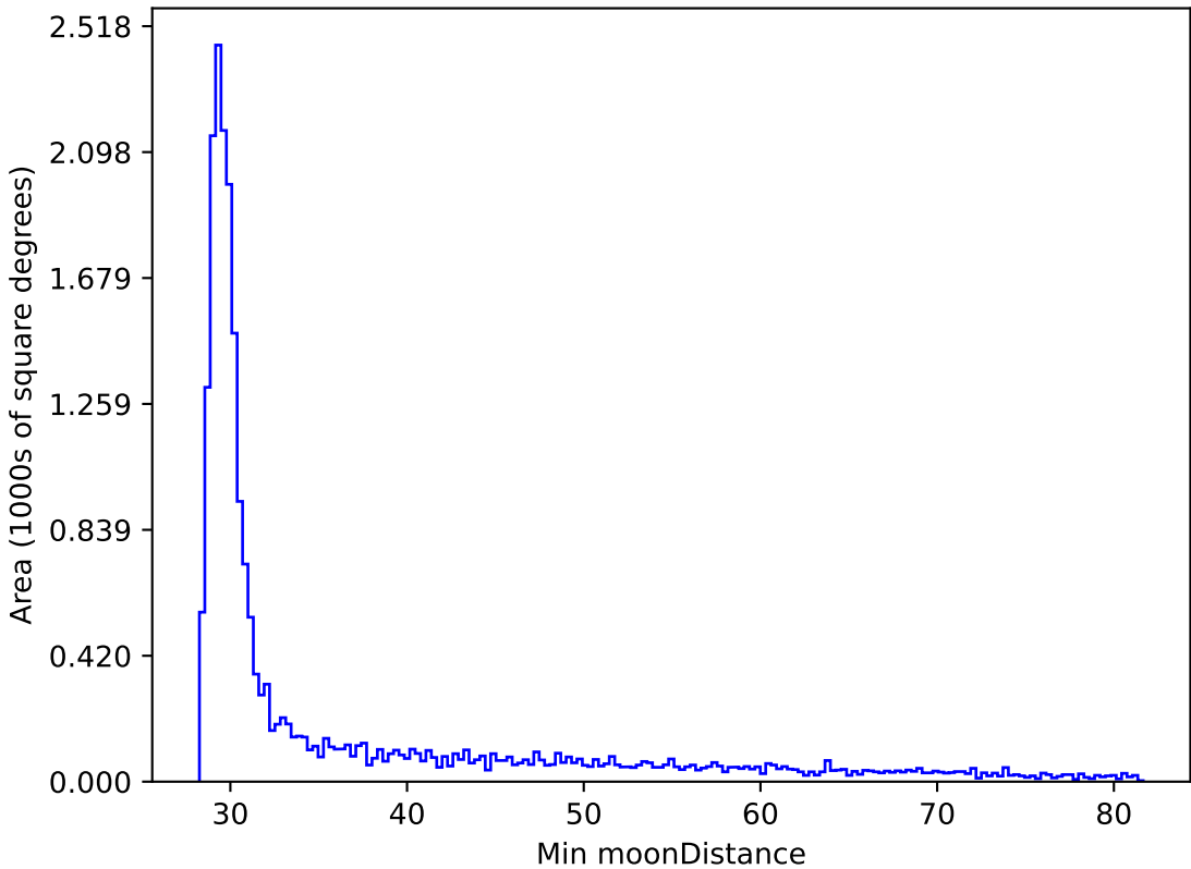
too_ignore_10_1v3.4_10yrs All sky y band: Min moonDistance
