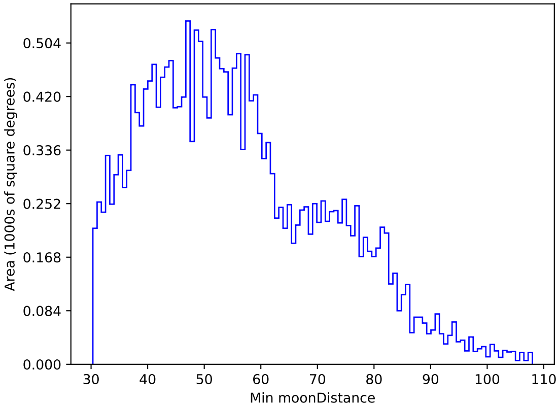
too_ignore_10_1v3.4_10yrs All sky u band: Min moonDistance
