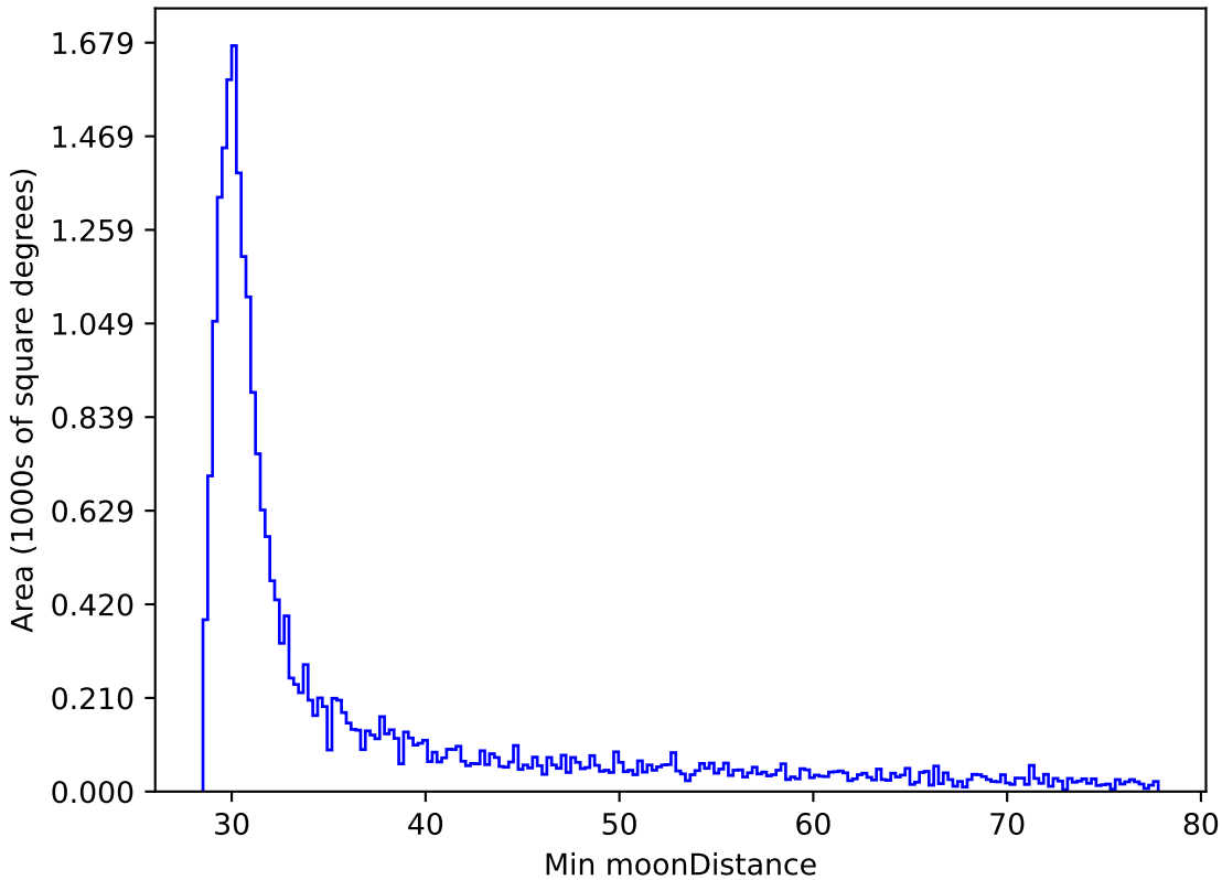
too_ignore_10_1v3.4_10yrs All sky i band: Min moonDistance
