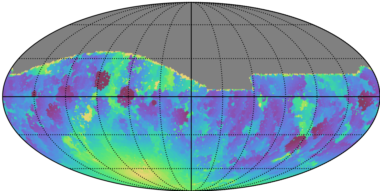
too_ignore_10_1v3.4_10yrs All sky g band: Min moonDistance
