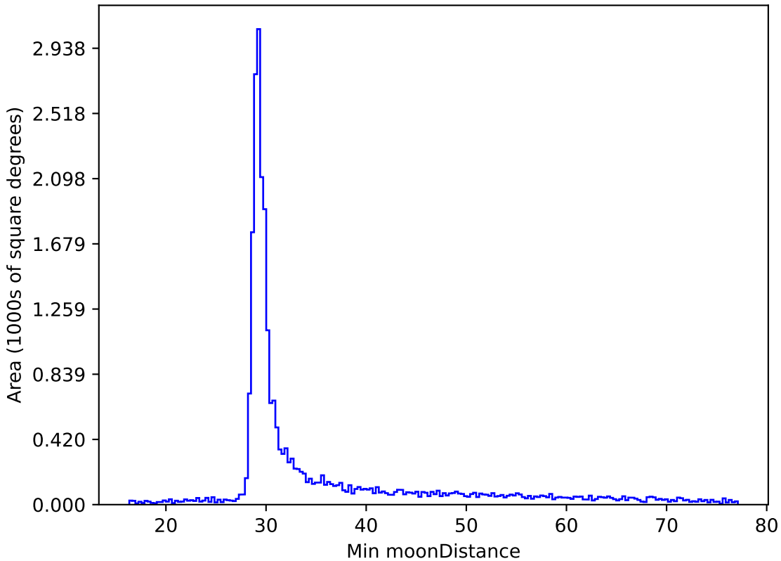
too_ignore_10_1v3.4_10yrs All sky all bands: Min moonDistance
