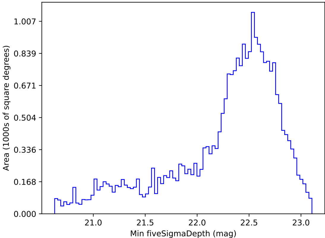
too_ignore_10_1v3.4_10yrs Yr 1 z band: Min fiveSigmaDepth
