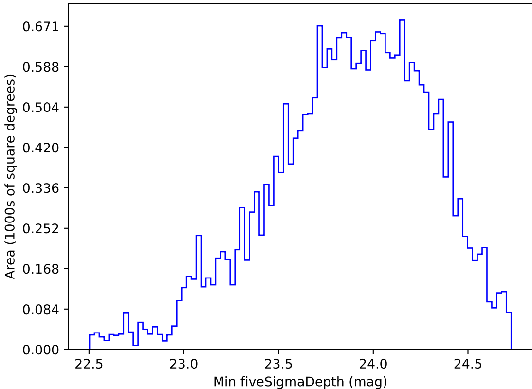
too_ignore_10_1v3.4_10yrs Yr 1 g band: Min fiveSigmaDepth
