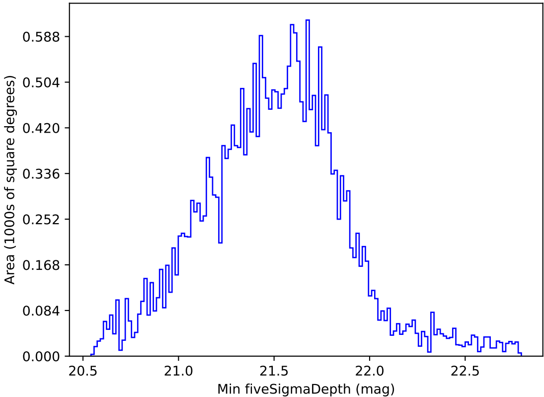
too_ignore_10_1v3.4_10yrs Yr 1 all bands: Min fiveSigmaDepth
