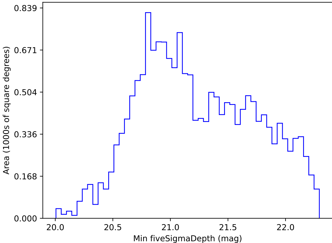
too_ignore_10_1v3.4_10yrs WFD z band: Min fiveSigmaDepth
