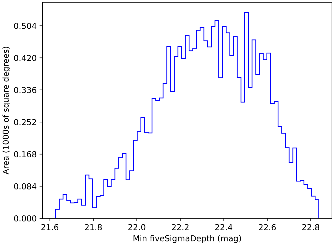
too_ignore_10_1v3.4_10yrs WFD u band: Min fiveSigmaDepth
