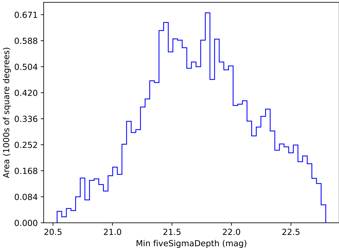
too_ignore_10_1v3.4_10yrs WFD i band: Min fiveSigmaDepth
