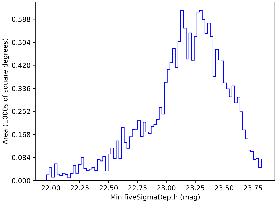
too_ignore_10_1v3.4_10yrs WFD g band: Min fiveSigmaDepth
