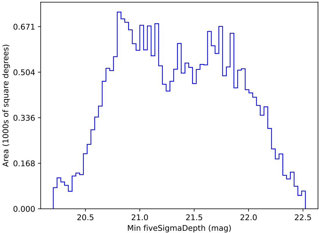
too_ignore_10_1v3.4_10yrs All sky z band: Min fiveSigmaDepth
