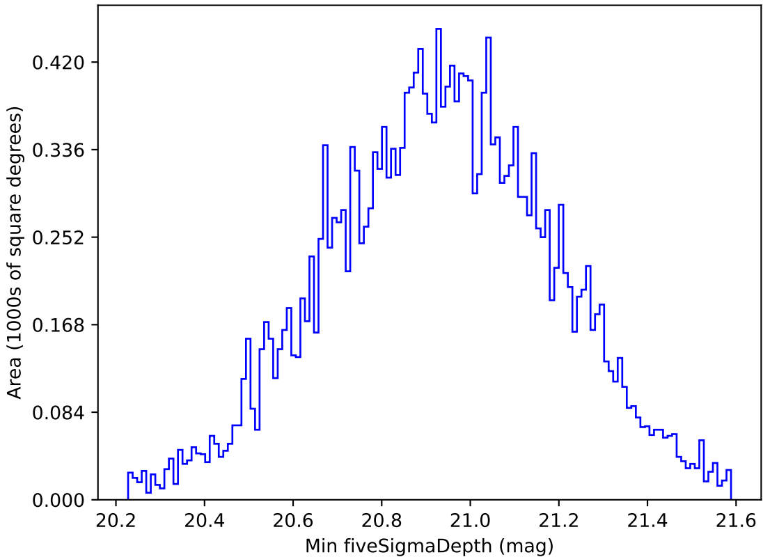
too_ignore_10_1v3.4_10yrs All sky y band: Min fiveSigmaDepth
