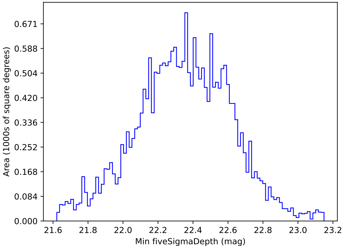
too_ignore_10_1v3.4_10yrs All sky u band: Min fiveSigmaDepth
