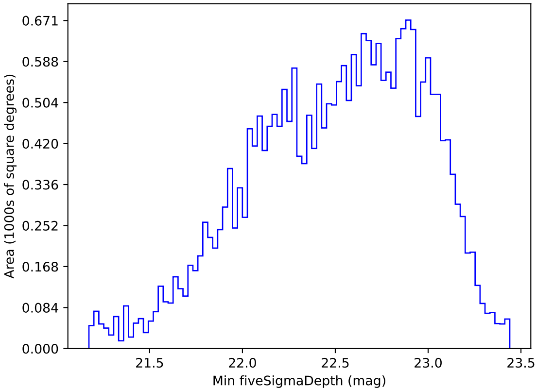
too_ignore_10_1v3.4_10yrs All sky r band: Min fiveSigmaDepth
