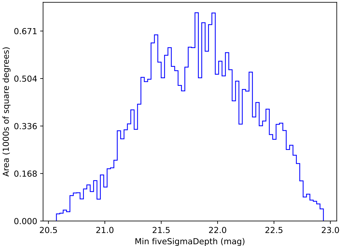
too_ignore_10_1v3.4_10yrs All sky i band: Min fiveSigmaDepth
