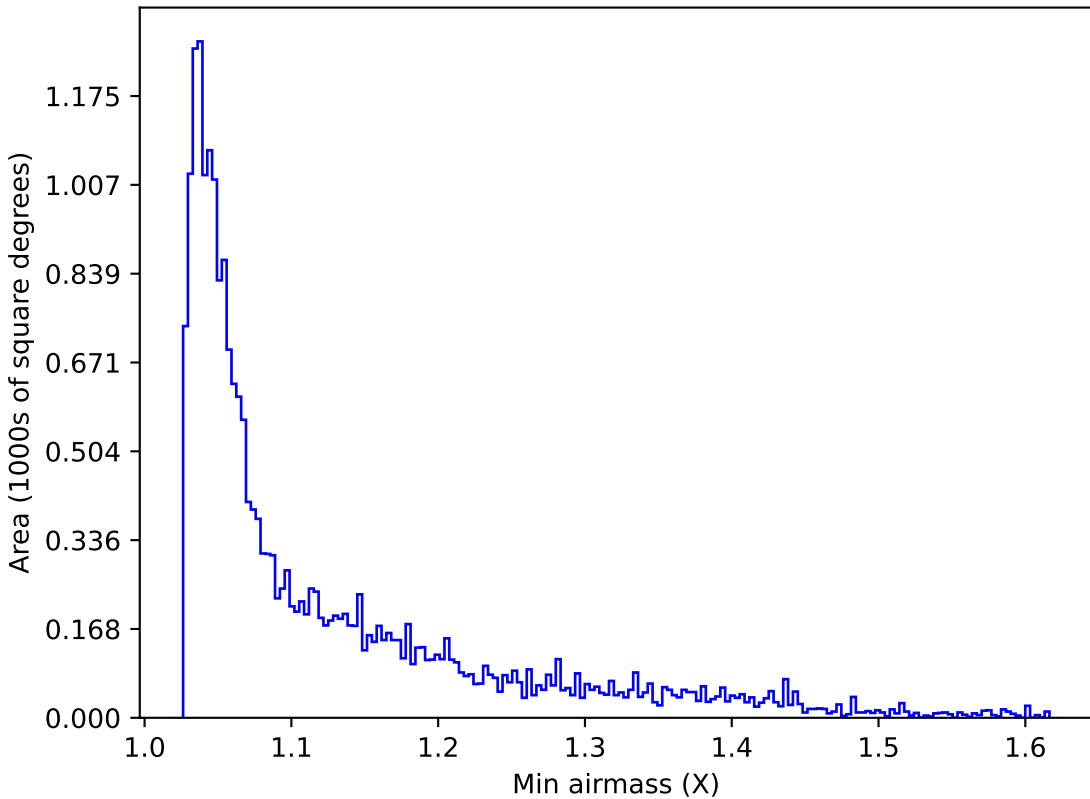
too_ignore_10_1v3.4_10yrs Yr 1 y band: Min airmass
