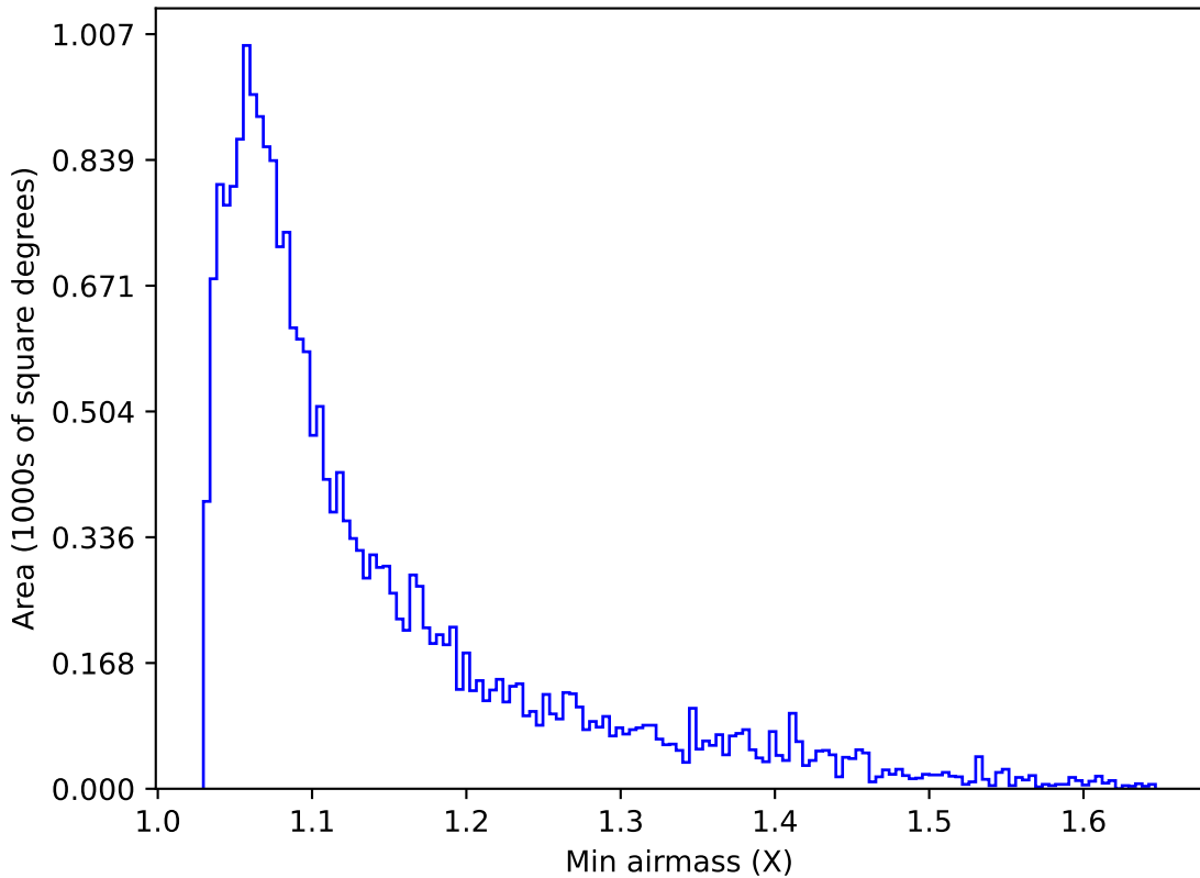
too_ignore_10_1v3.4_10yrs Yr 1 u band: Min airmass
