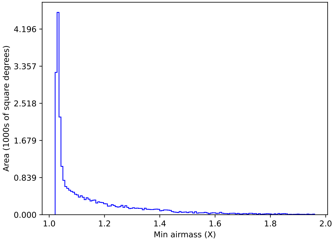
too_ignore_10_1v3.4_10yrs Yr 1 all bands: Min airmass
