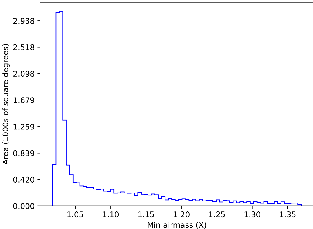
too_ignore_10_1v3.4_10yrs WFD z band: Min airmass
