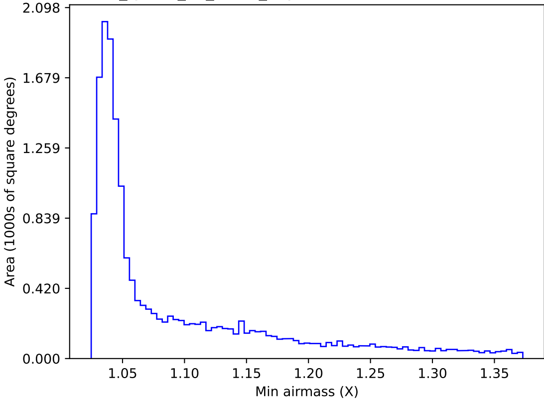
too_ignore_10_1v3.4_10yrs WFD u band: Min airmass
