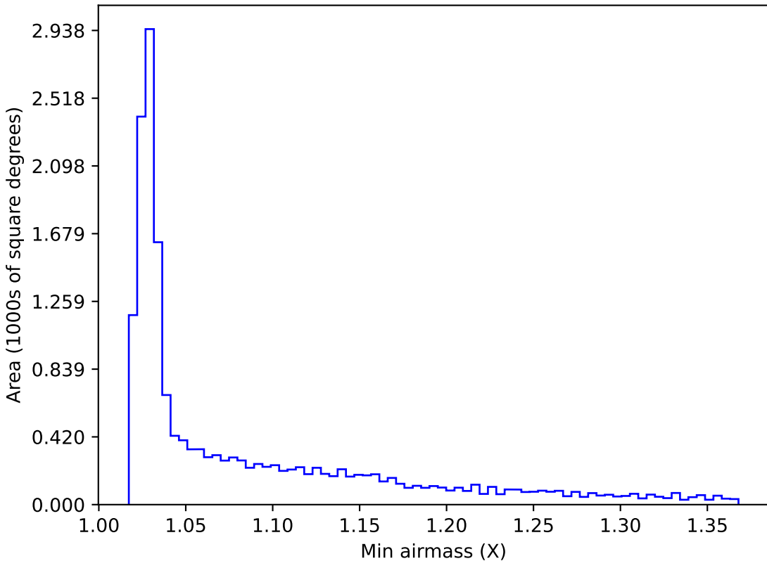
too_ignore_10_1v3.4_10yrs WFD r band: Min airmass
