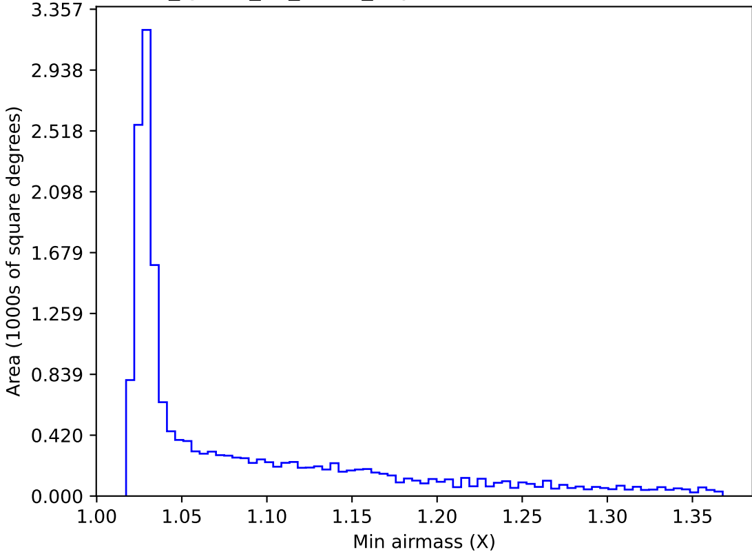
too_ignore_10_1v3.4_10yrs WFD i band: Min airmass
