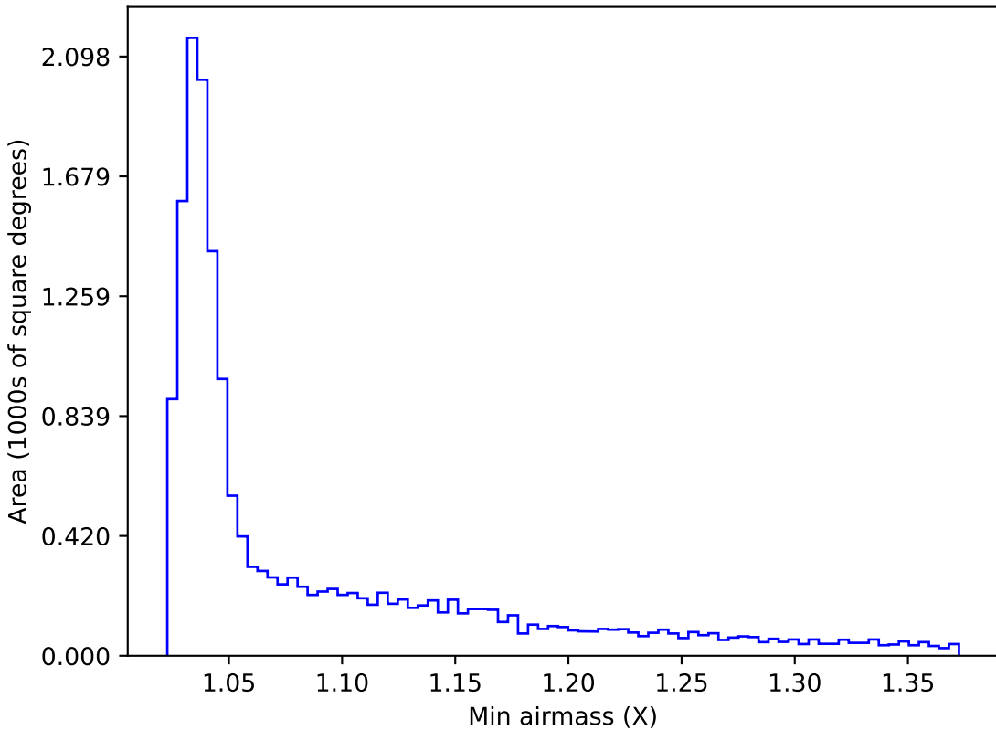
too_ignore_10_1v3.4_10yrs WFD g band: Min airmass
