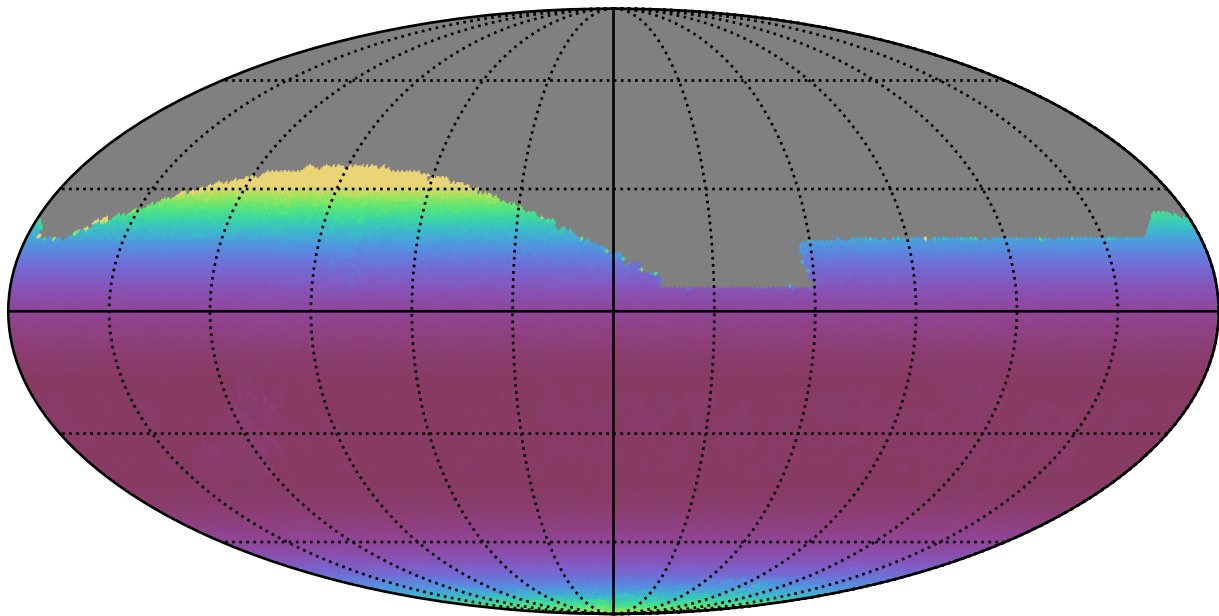
too_ignore_10_1v3.4_10yrs All sky z band: Min airmass
