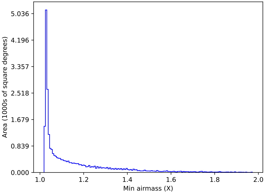
too_ignore_10_1v3.4_10yrs All sky z band: Min airmass
