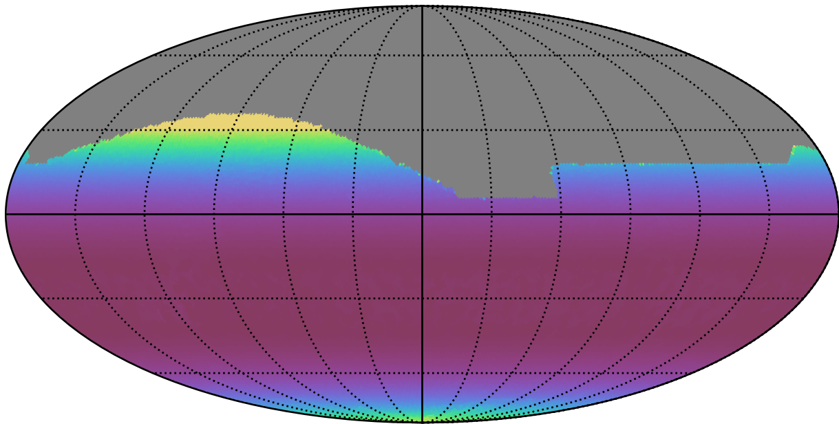
too_ignore_10_1v3.4_10yrs All sky r band: Min airmass
