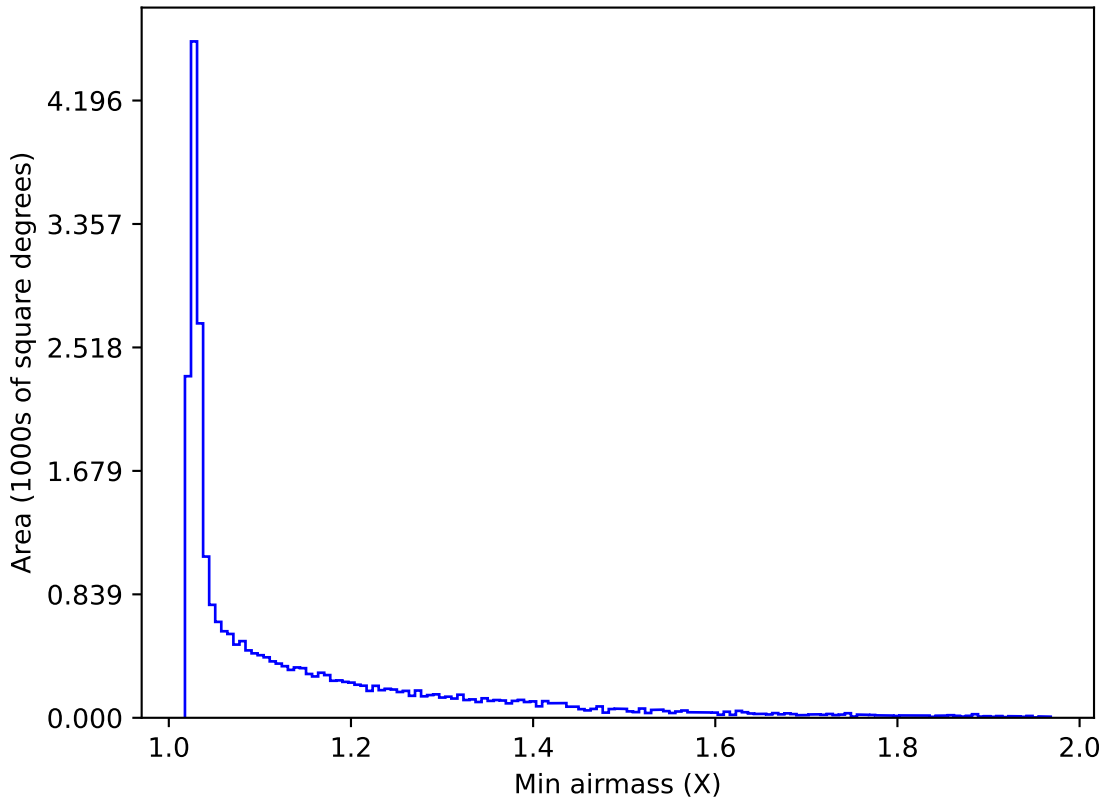
too_ignore_10_1v3.4_10yrs All sky r band: Min airmass
