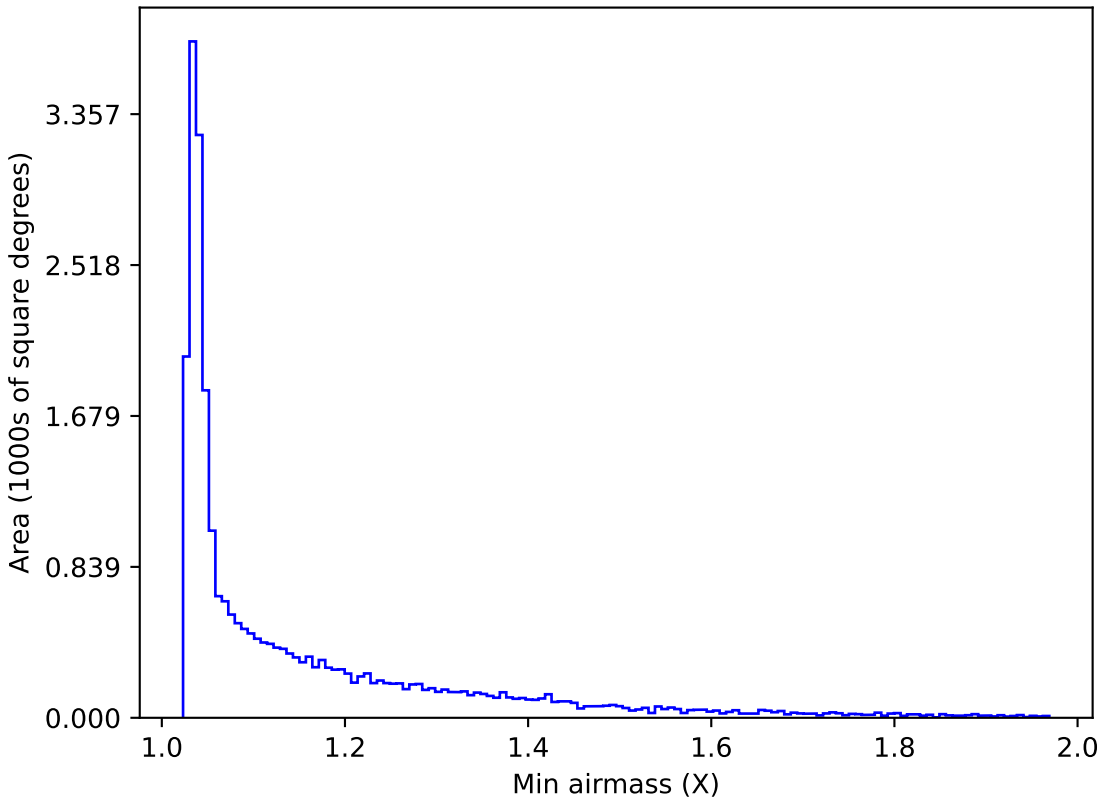
too_ignore_10_1v3.4_10yrs All sky g band: Min airmass
