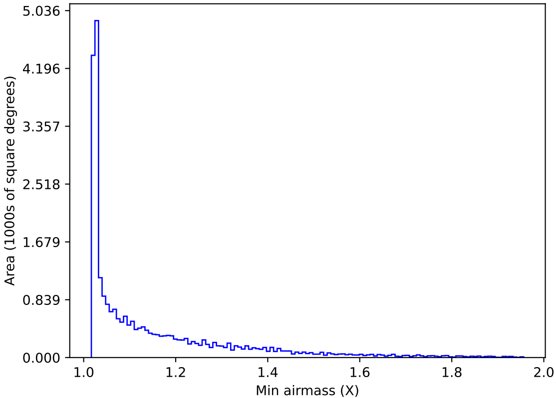
too_ignore_10_1v3.4_10yrs All sky all bands: Min airmass
