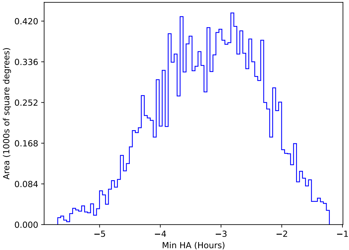
too_ignore_10_1v3.4_10yrs WFD u band: Min HA
