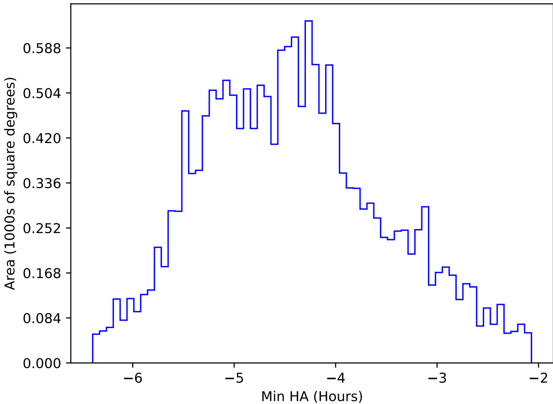
too_ignore_10_1v3.4_10yrs WFD r band: Min HA
