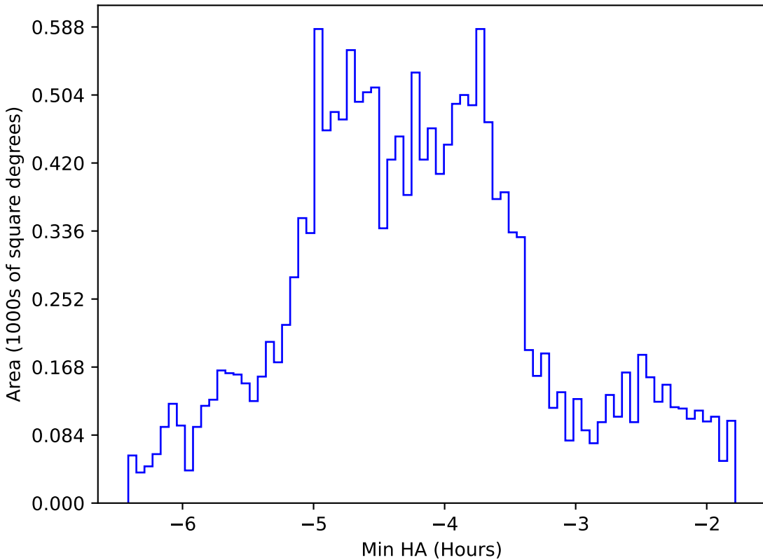
too_ignore_10_1v3.4_10yrs WFD g band: Min HA
