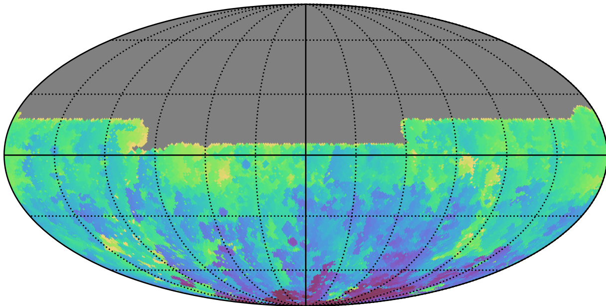
too_ignore_10_1v3.4_10yrs All sky u band: Min HA
