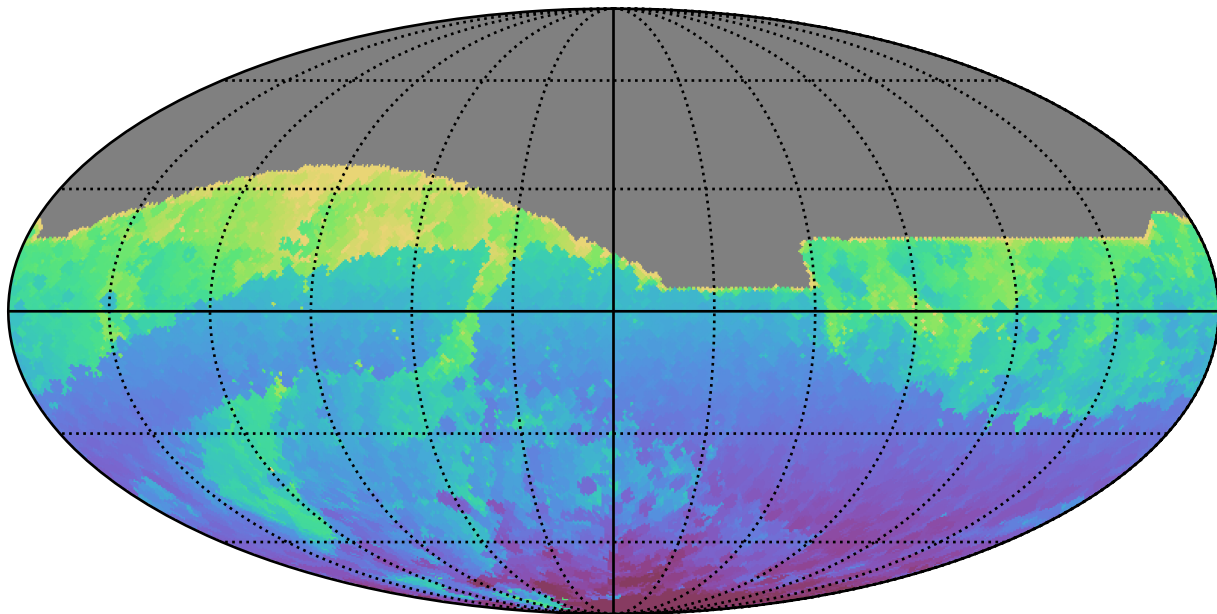
too_ignore_10_1v3.4_10yrs All sky r band: Min HA
