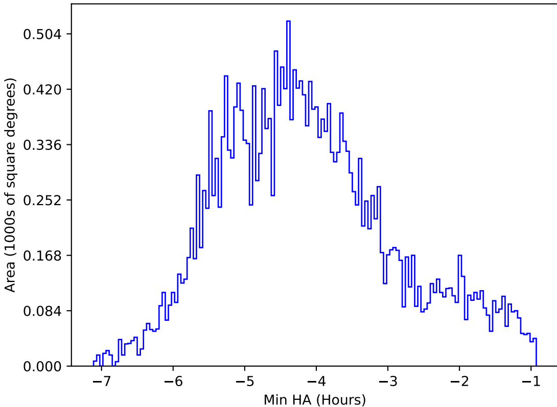
too_ignore_10_1v3.4_10yrs All sky r band: Min HA
